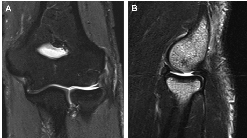
Figure 4 Magnetic resonance imaging investigation showing elbow plica observed on coronal T2 (A) and sagittal T1 (B) sequences.
